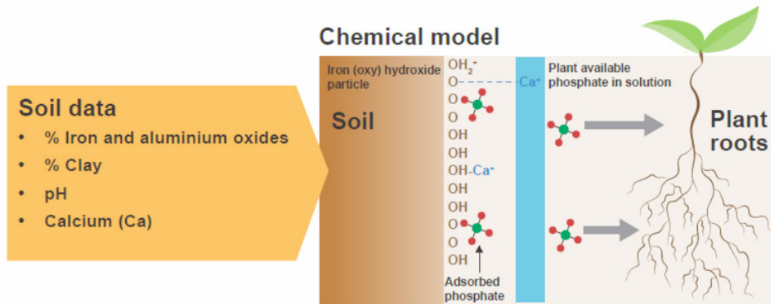
Fig. 1: Chemical model.
